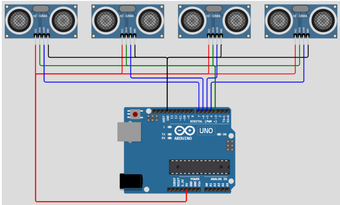
Figure 4.3.5: Circuit for Sensors
